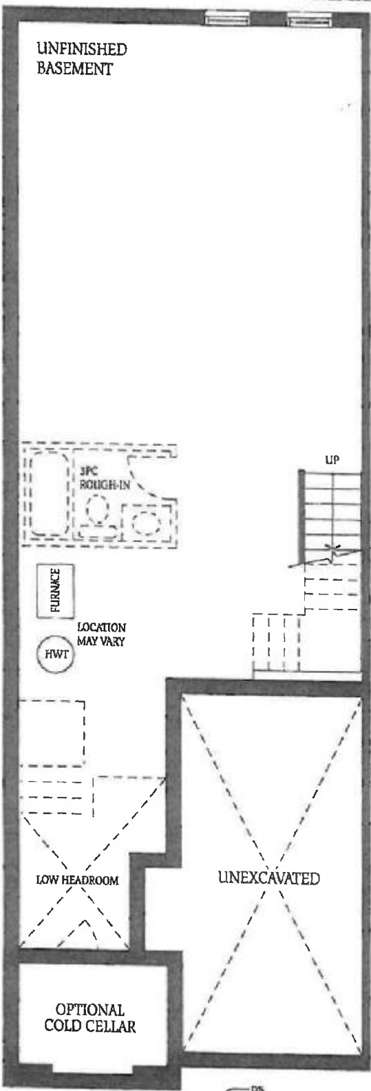
Basement Elevation A & B
