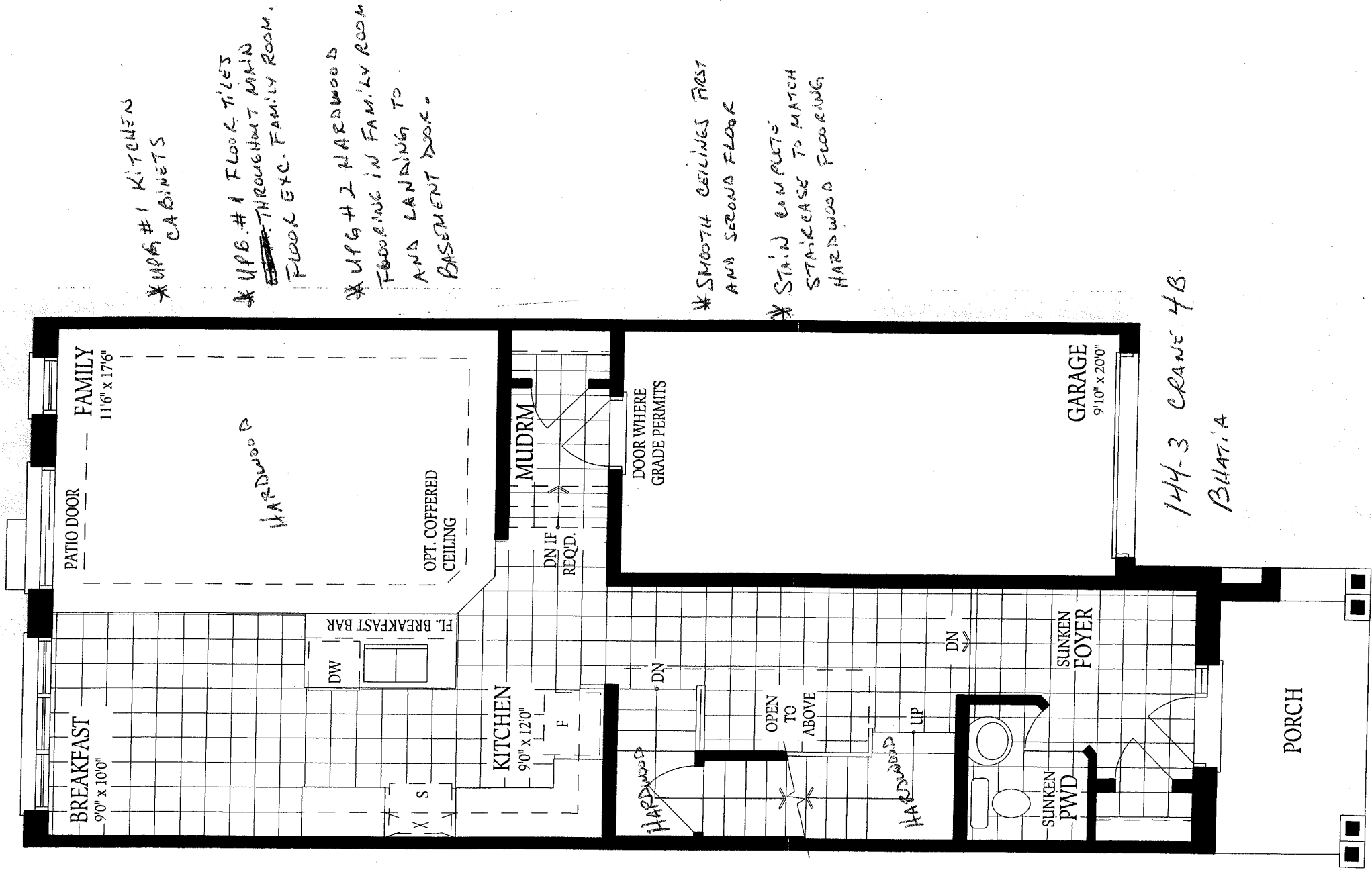
GROUND FLOOR ELEVATION B
