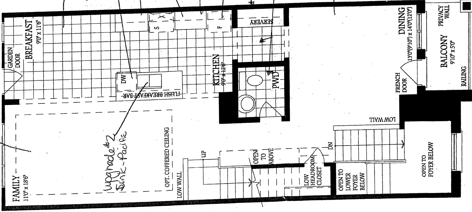
MAIN FLOOR ELEVATION A/A2/A3
