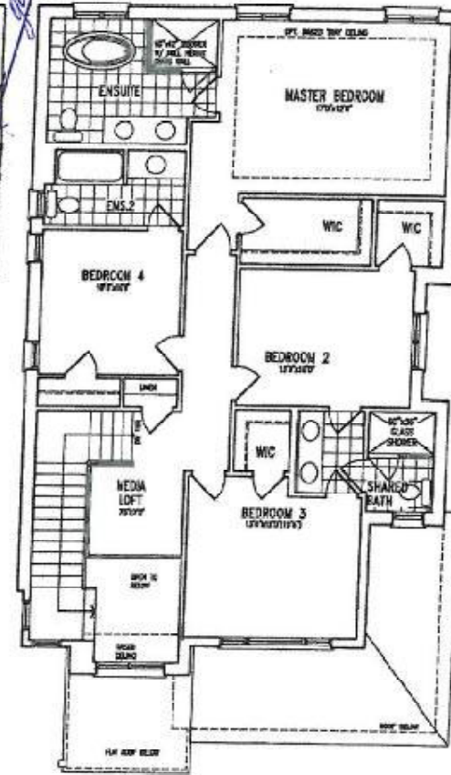
SECOND FLOOR PLAN 'C'
