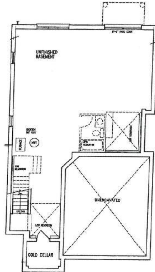
BASEMENT PLAN 'C'
