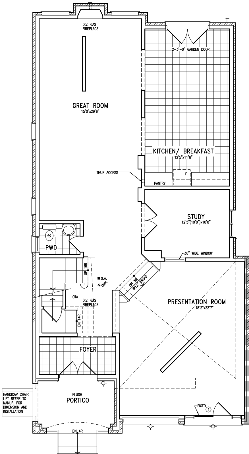
38-6 GROUND FLOOR PLAN 'B'
