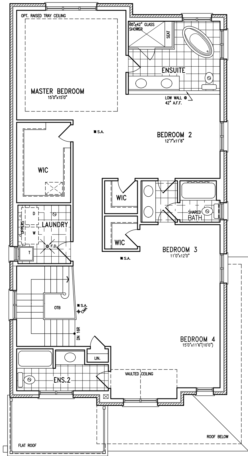
38-6 SECOND FLOOR PLAN 'B'
