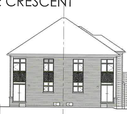
LOT # 69R - REAR ELEVATION SD25-4C -EL. C (REV.)
