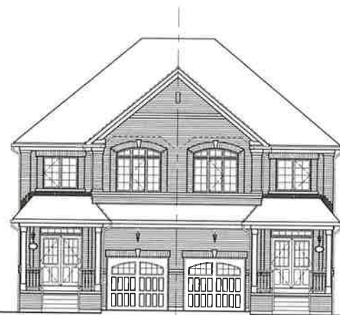
LOT # 65L - FRONT ELEVATION SD25-4 -EL. A
