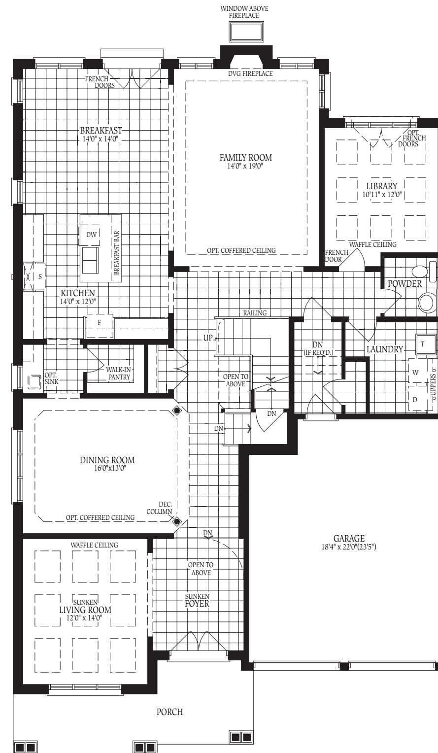
GROUND FLOOR PLAN 'B'
