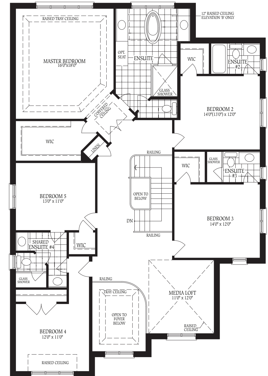
SECOND FLOOR PLAN 'B'
