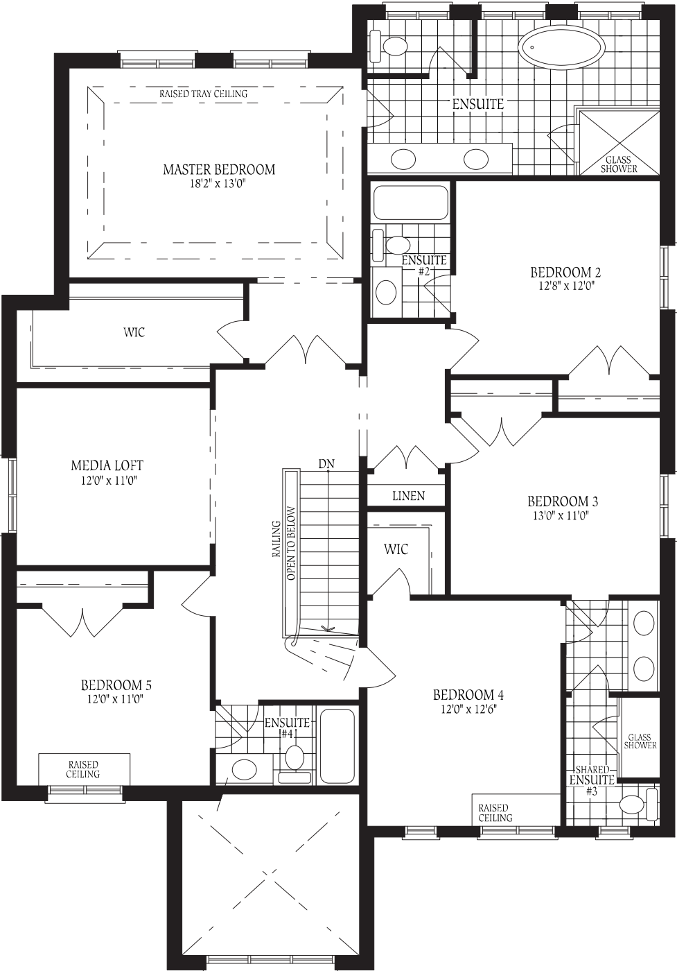
SECOND FLOOR 'B'
