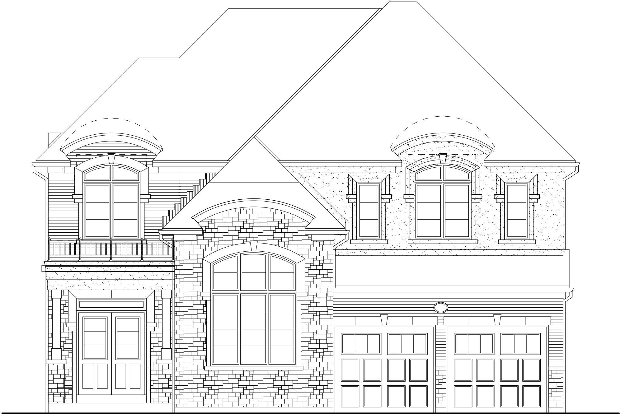
LOT 187 FRONT ELEVATION 'B'
