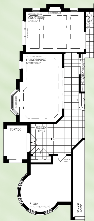
Ground Floor Elevation B
