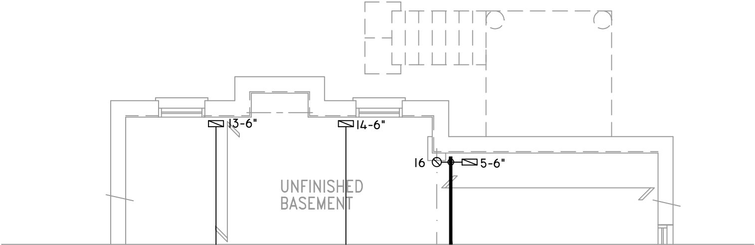
PARTIAL BASEMENT PLAN W.O.D. 9R AND MORE CONDITION ELEV. 'A'
