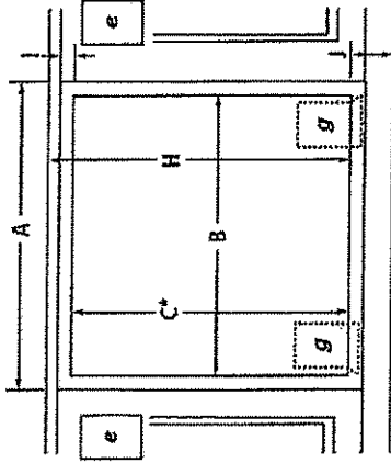
UNDER COUNTER INSTALLATION (without cooktop installed above)
