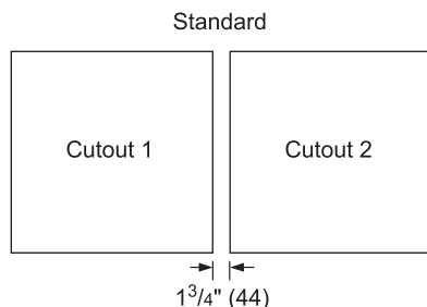
Side-by-Side Installation
