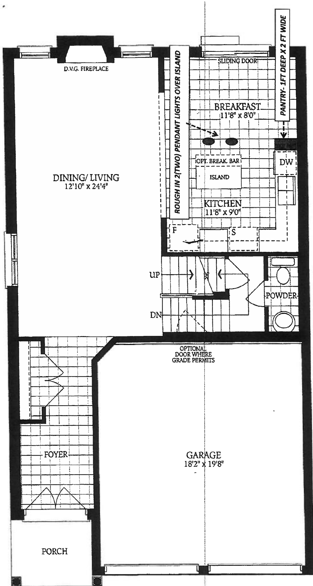
Main Level - Elevation A
