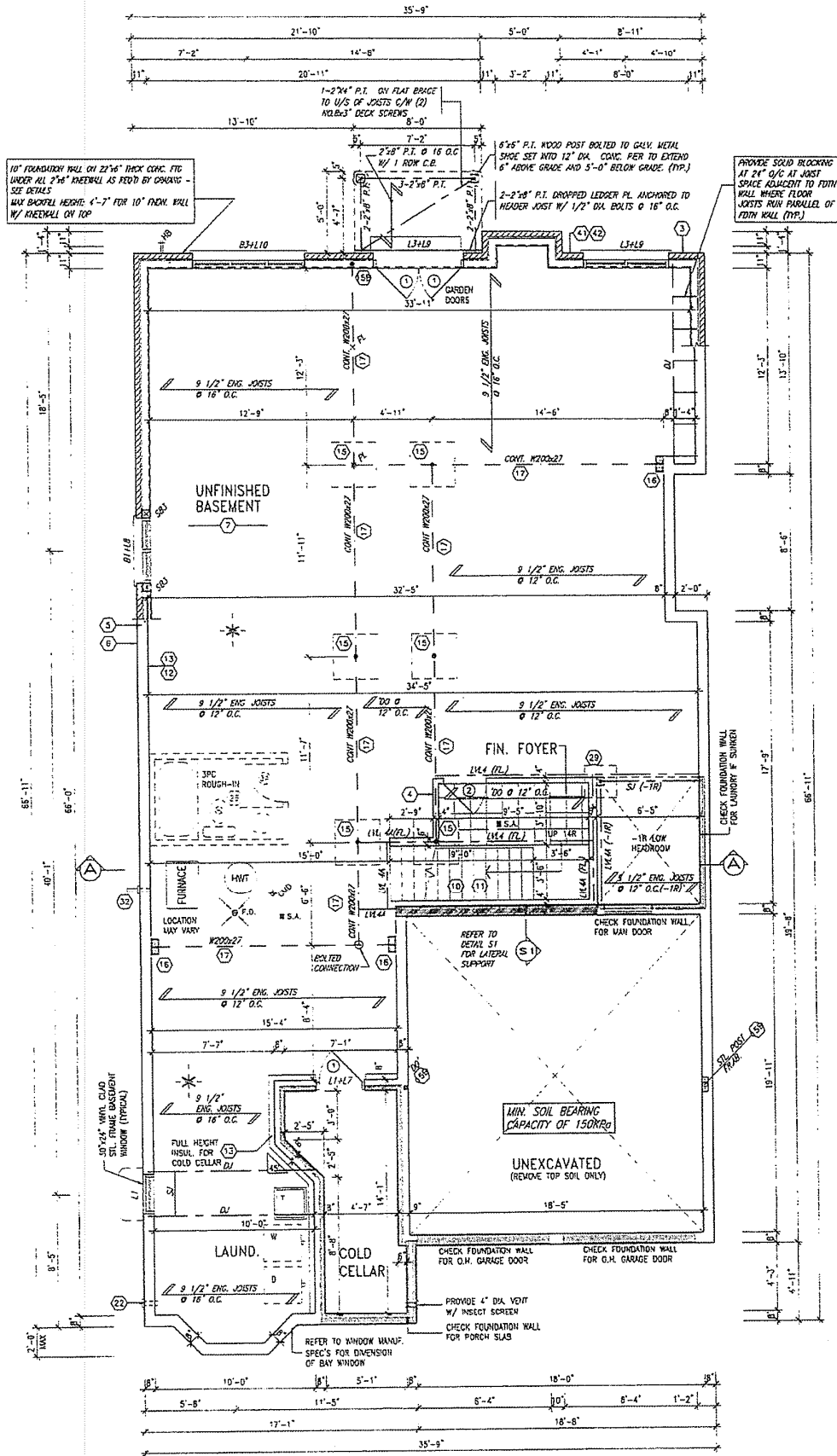
BASEMENT PLAN - ELEV. 'B'
