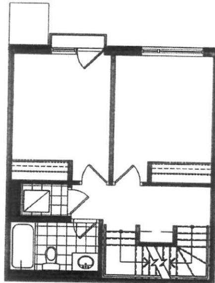
2ND FLOOR
