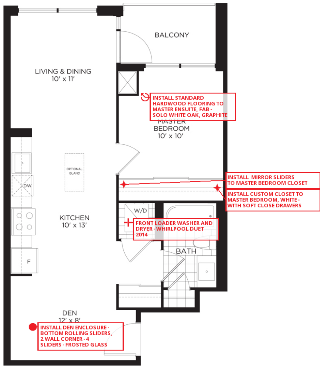
MAIN LEVEL
