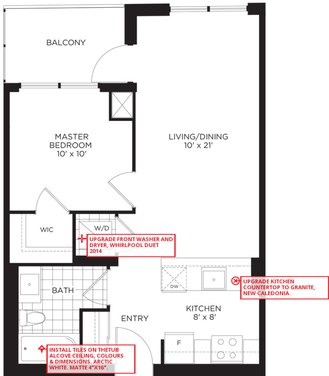
MAIN LEVEL
