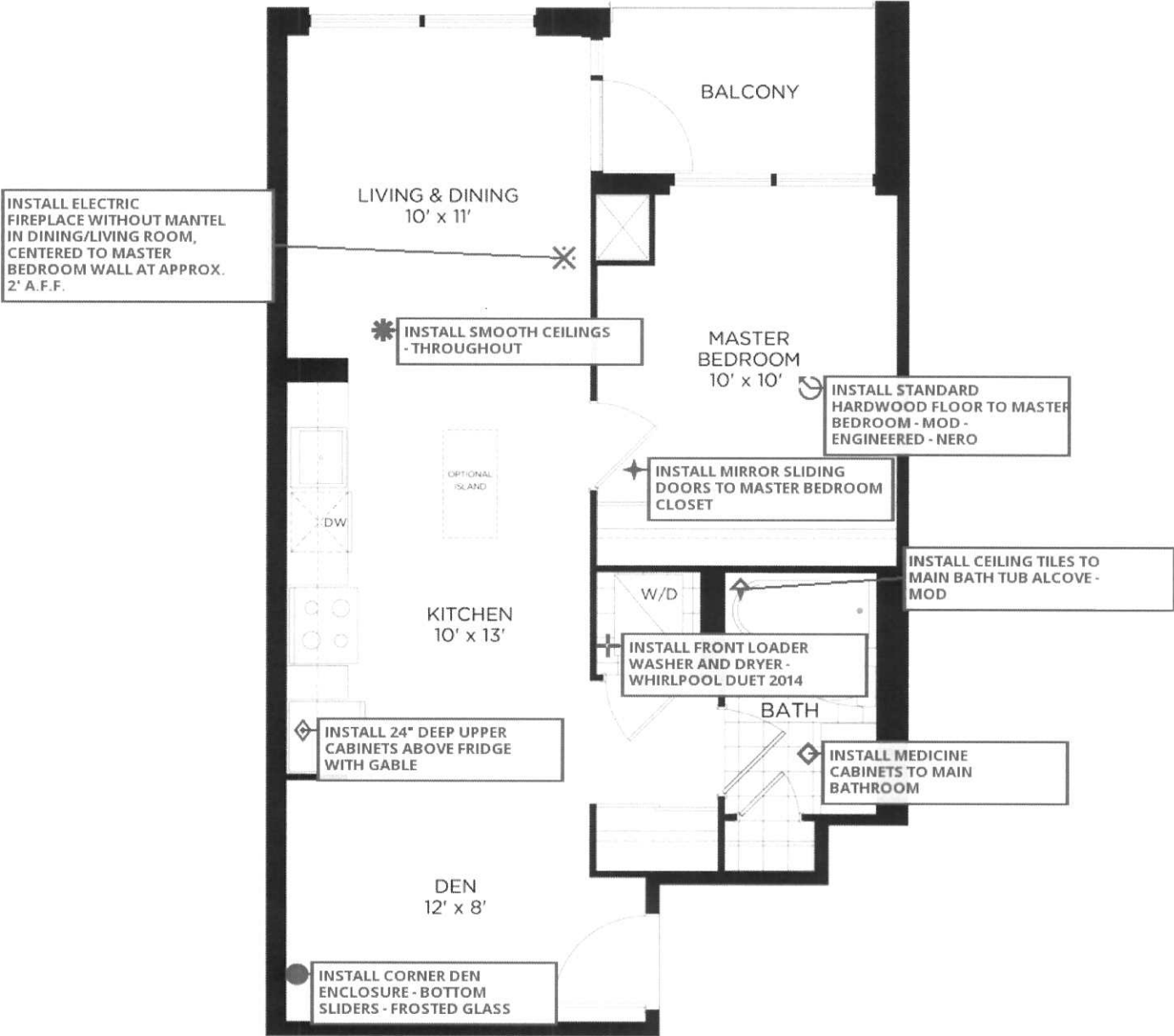
MAIN LEVEL
