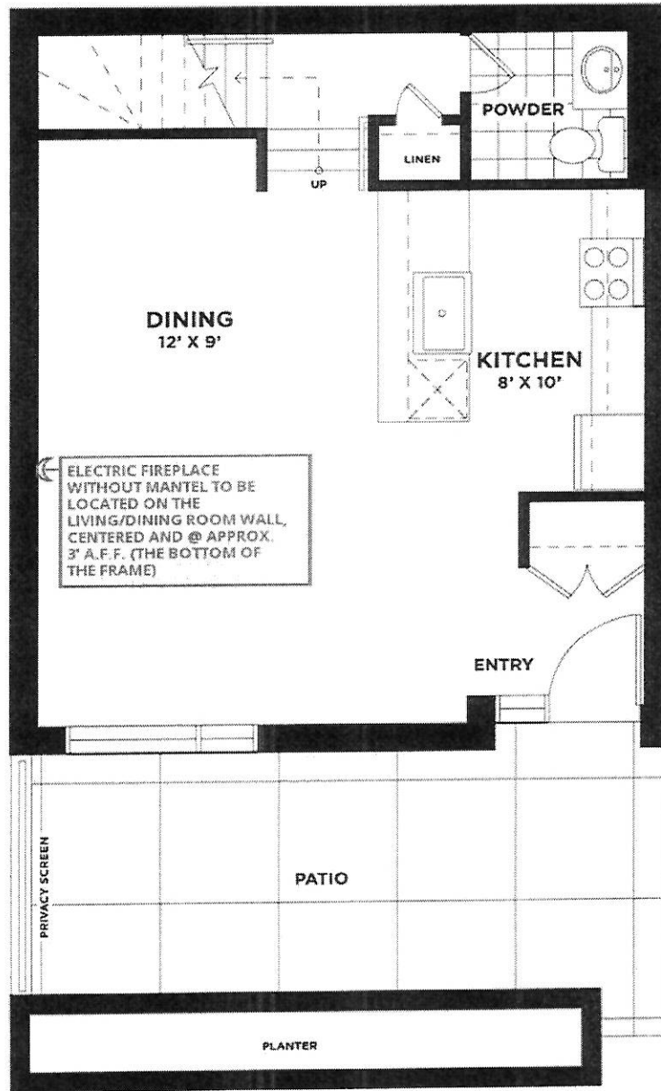
GROUND LEVEL
