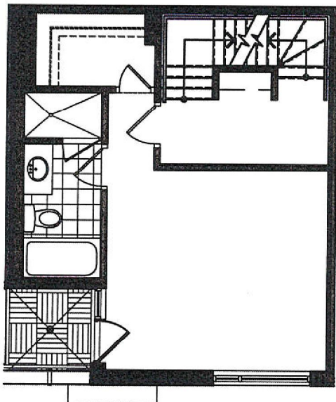
3RD FLOOR
