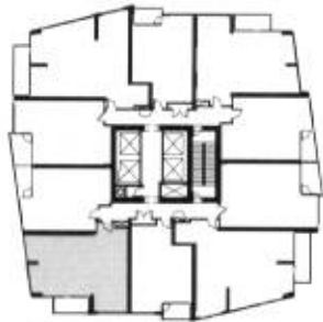
TYPICAL FLOOR
