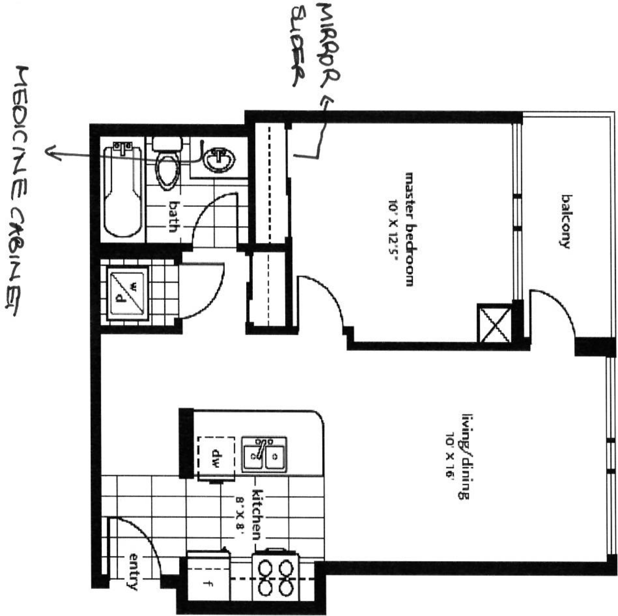
Floor Plan: 1
