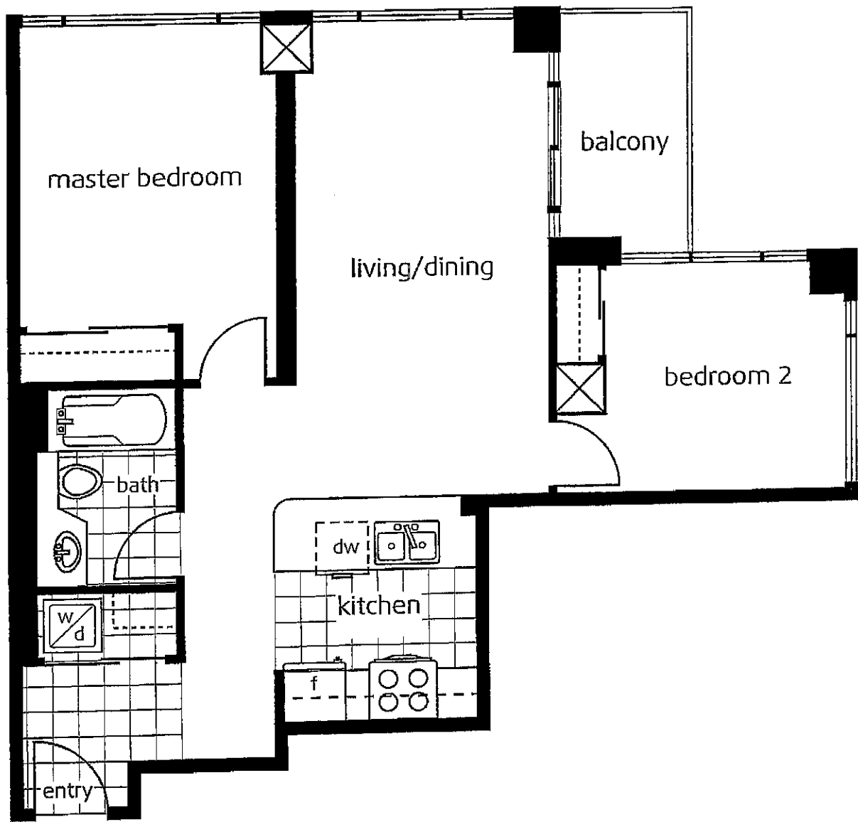
floorplan 11:
